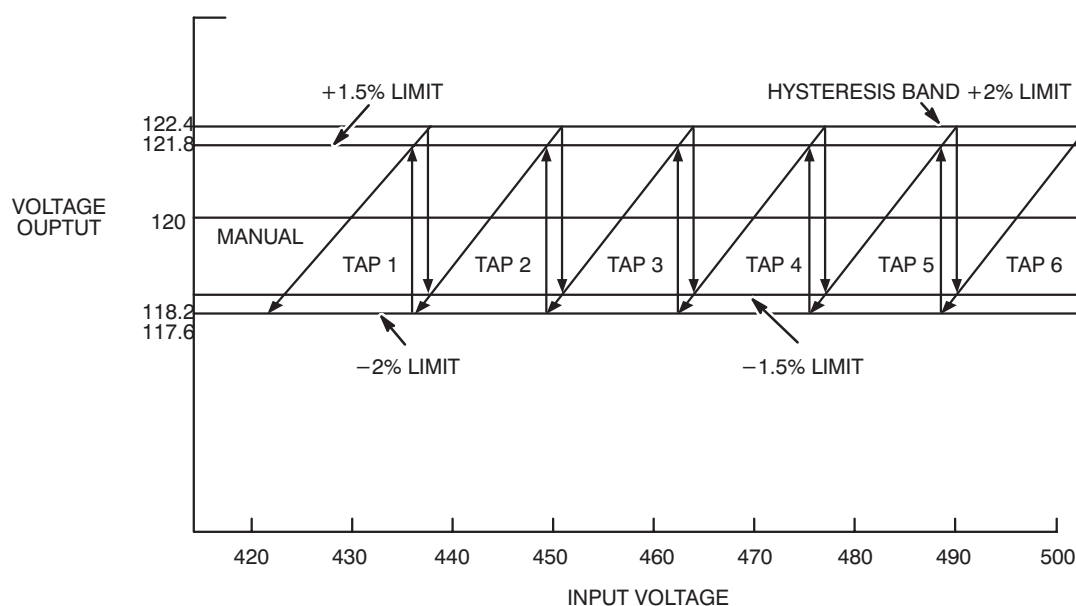
REGULATOR OUTPUT ACCURACY ILLUSTRATION 4-2
