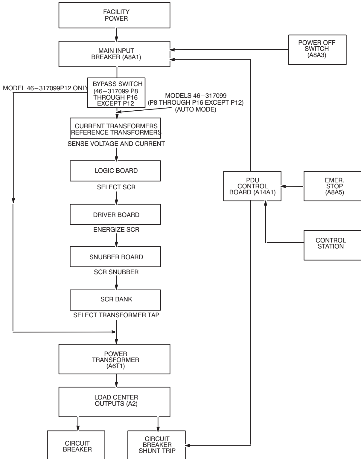
COMPACT PDU BLOCK DIAGRAM
